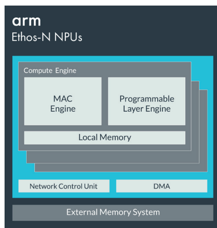
Ethos-N57 mainstream ML inference processor contains eight engines
