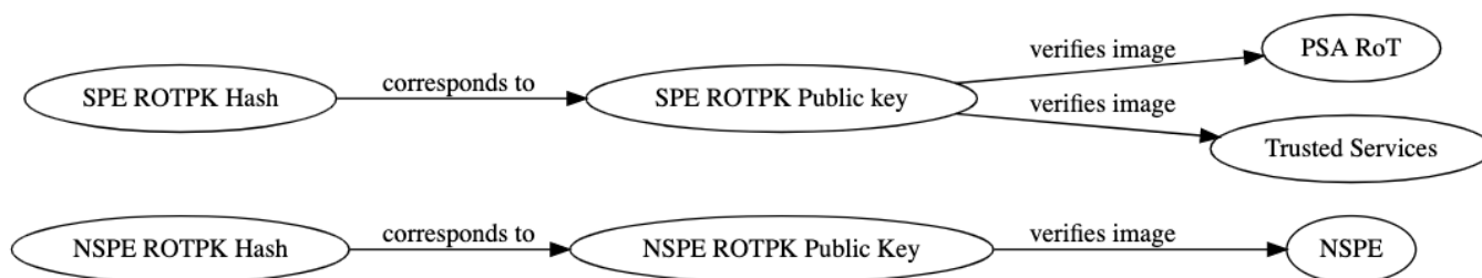
Figure 6: Example of multiple providers with independent roots of trust
