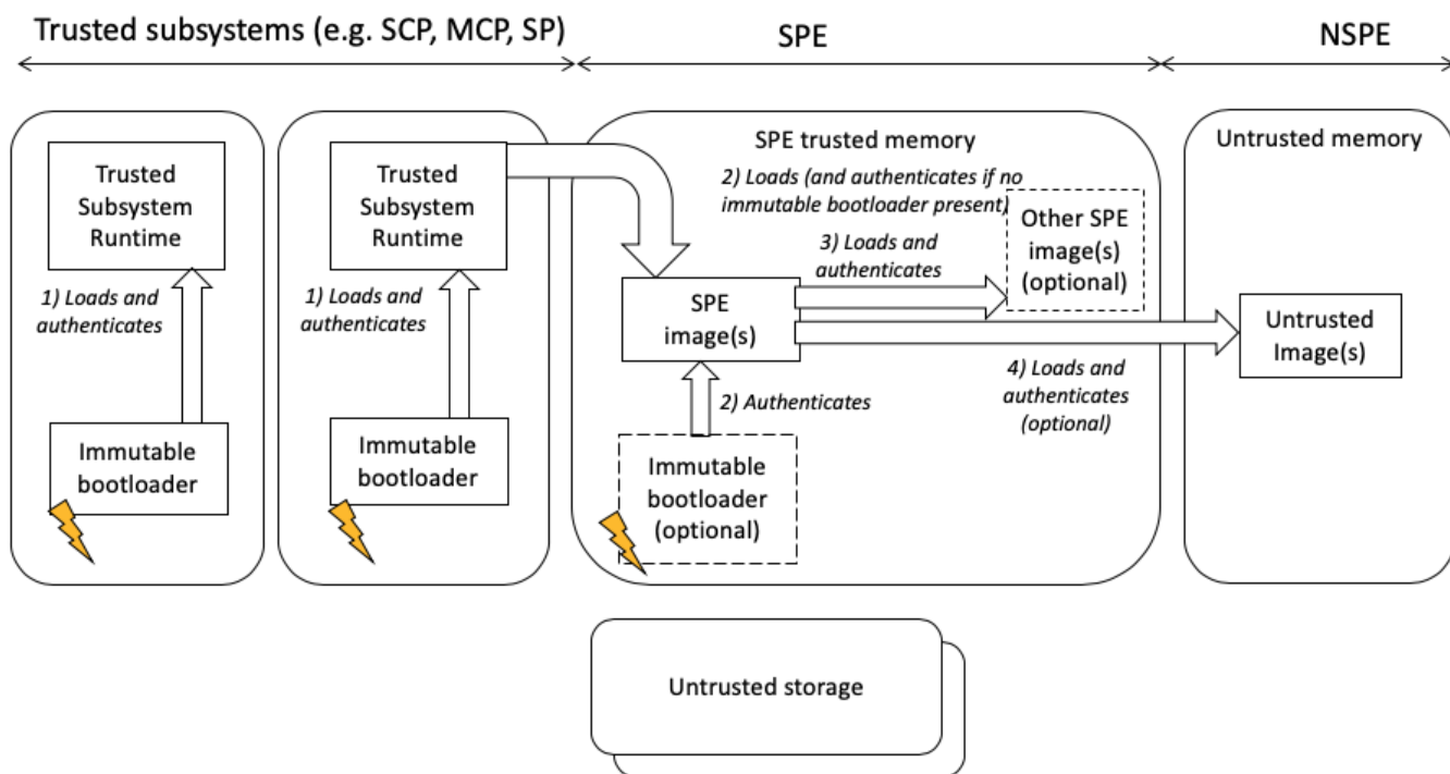
Figure 10: Example boot using a trusted subsystem that directly loads and verifies images in the SPE
