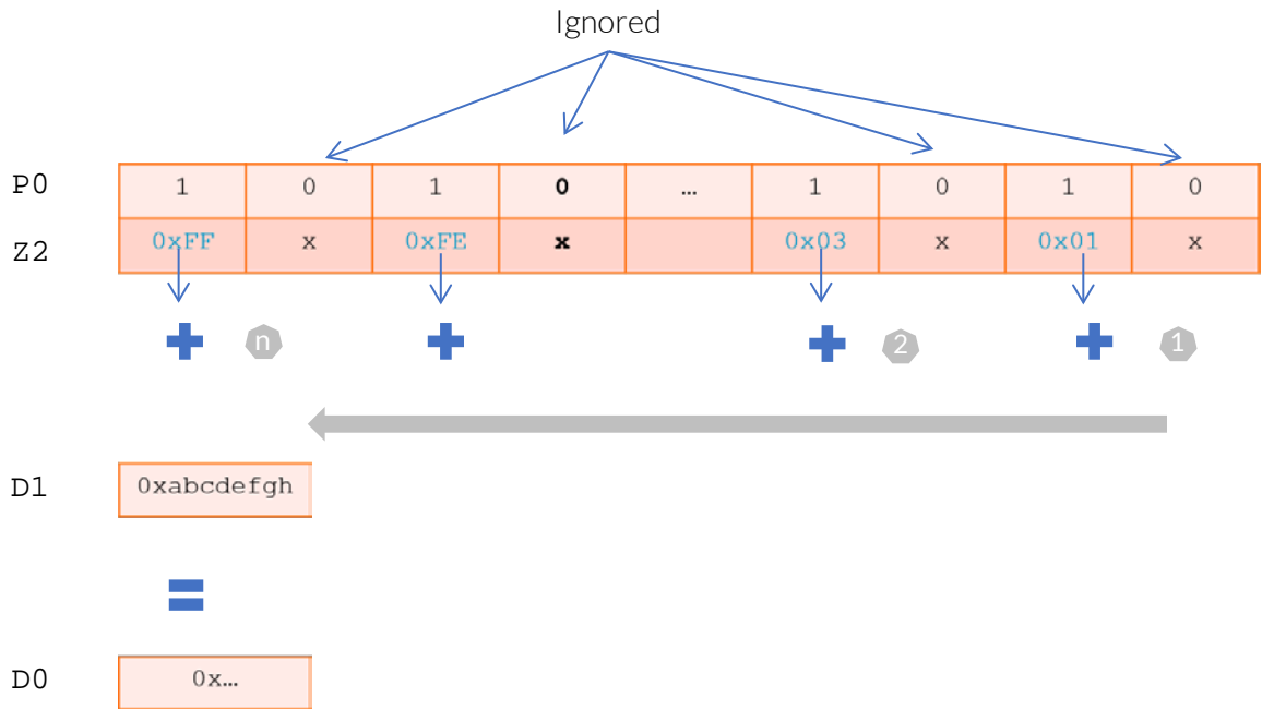
Figure 9 Extended floating-point and horizontal reductions example
