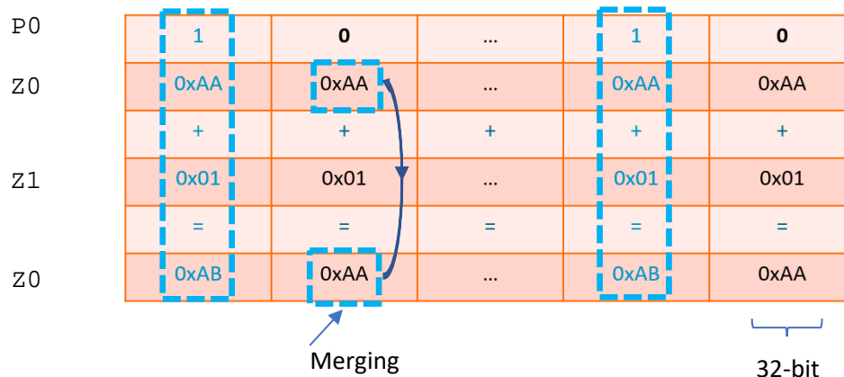
Figure 4 Per-lane predication merging
