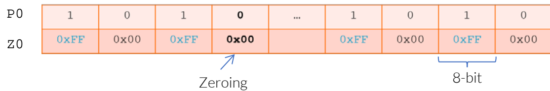
Figure 5 Per-lane predication zeroing
