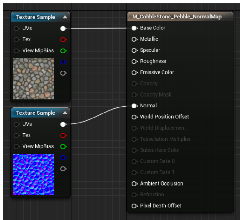
Fig. 21 - Adding a normal map texture in Unreal Engine
