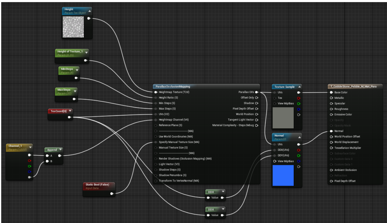
Fig. 22 - Parallax occlusion mapping material in Unreal Engine
