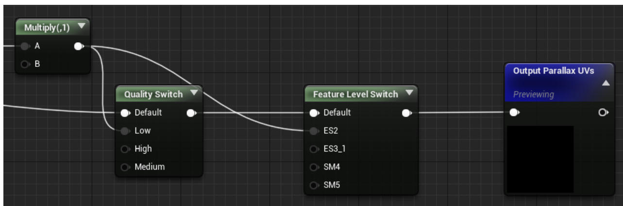
Fig. 23 - Parallax occlusion mapping node modification in Unreal Engine
