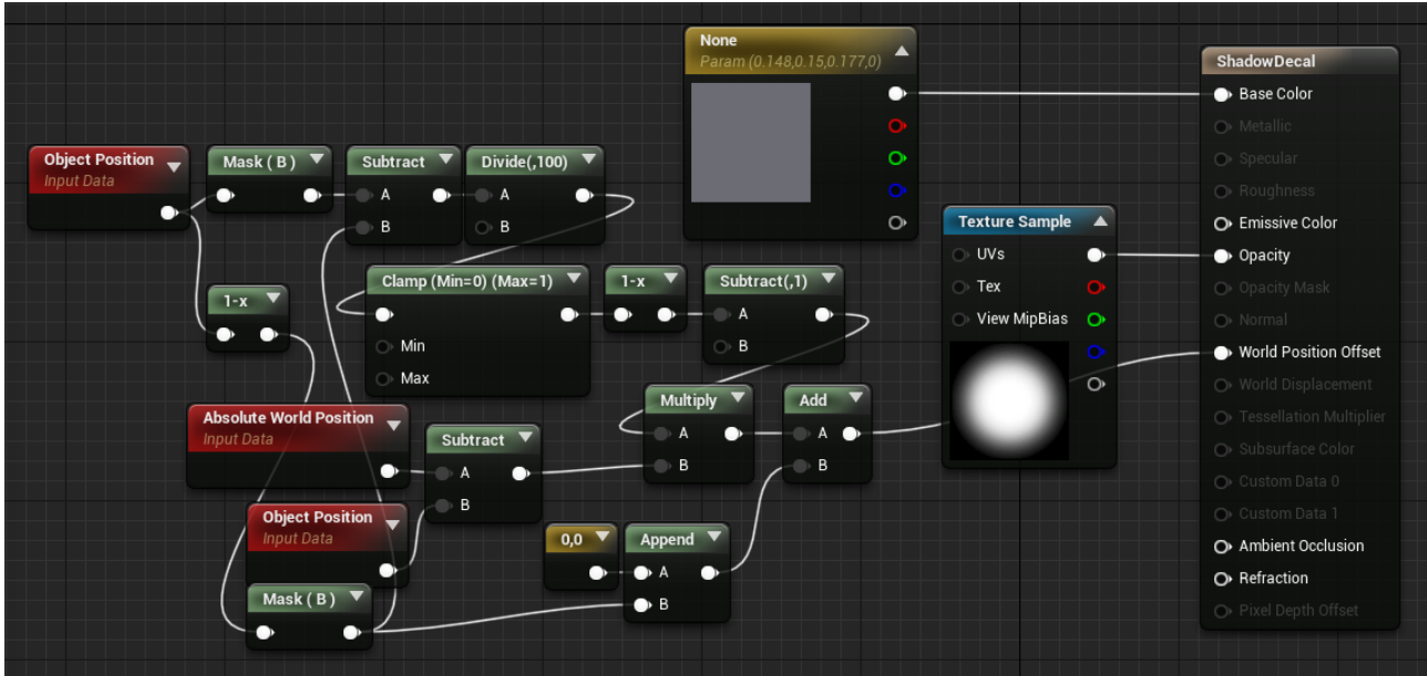
Fig. 25 - Blob shadow material in Unreal Engine
