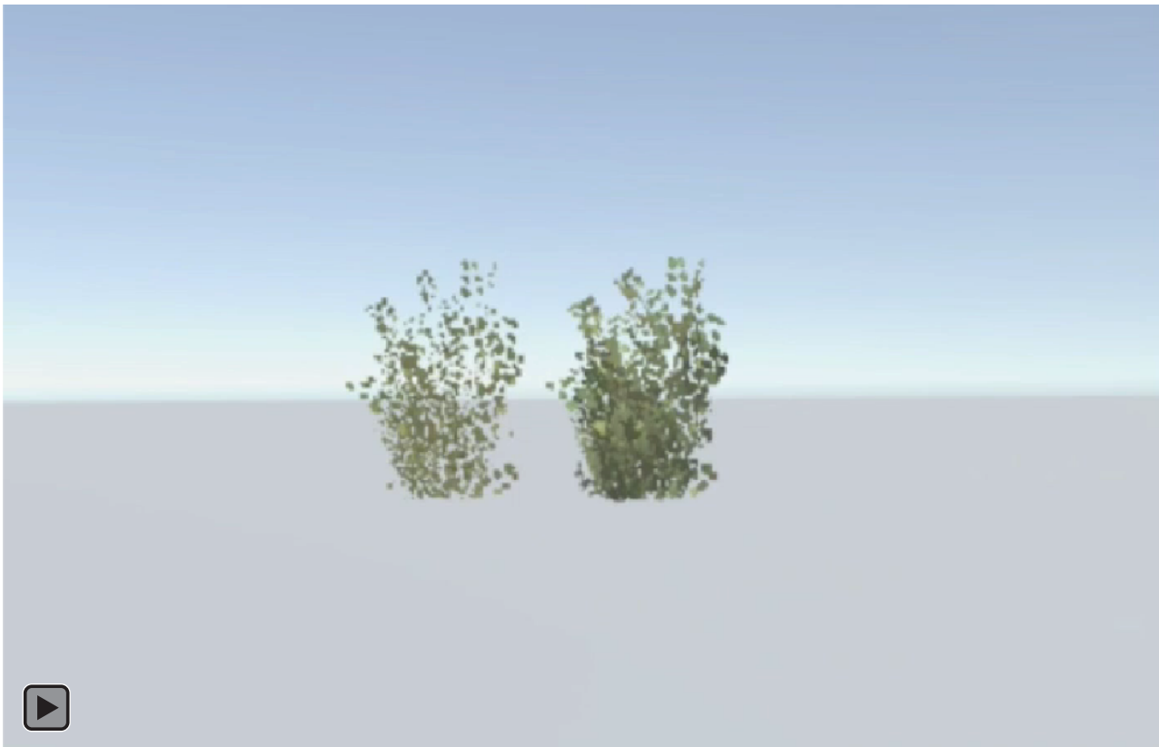
Fig. 13 - Video demonstrating alpha testing (left) and alpha to coverage (right) If this video does not load, please click here: https://www.youtube.com/watch?v=9nBprtPhXEQ
